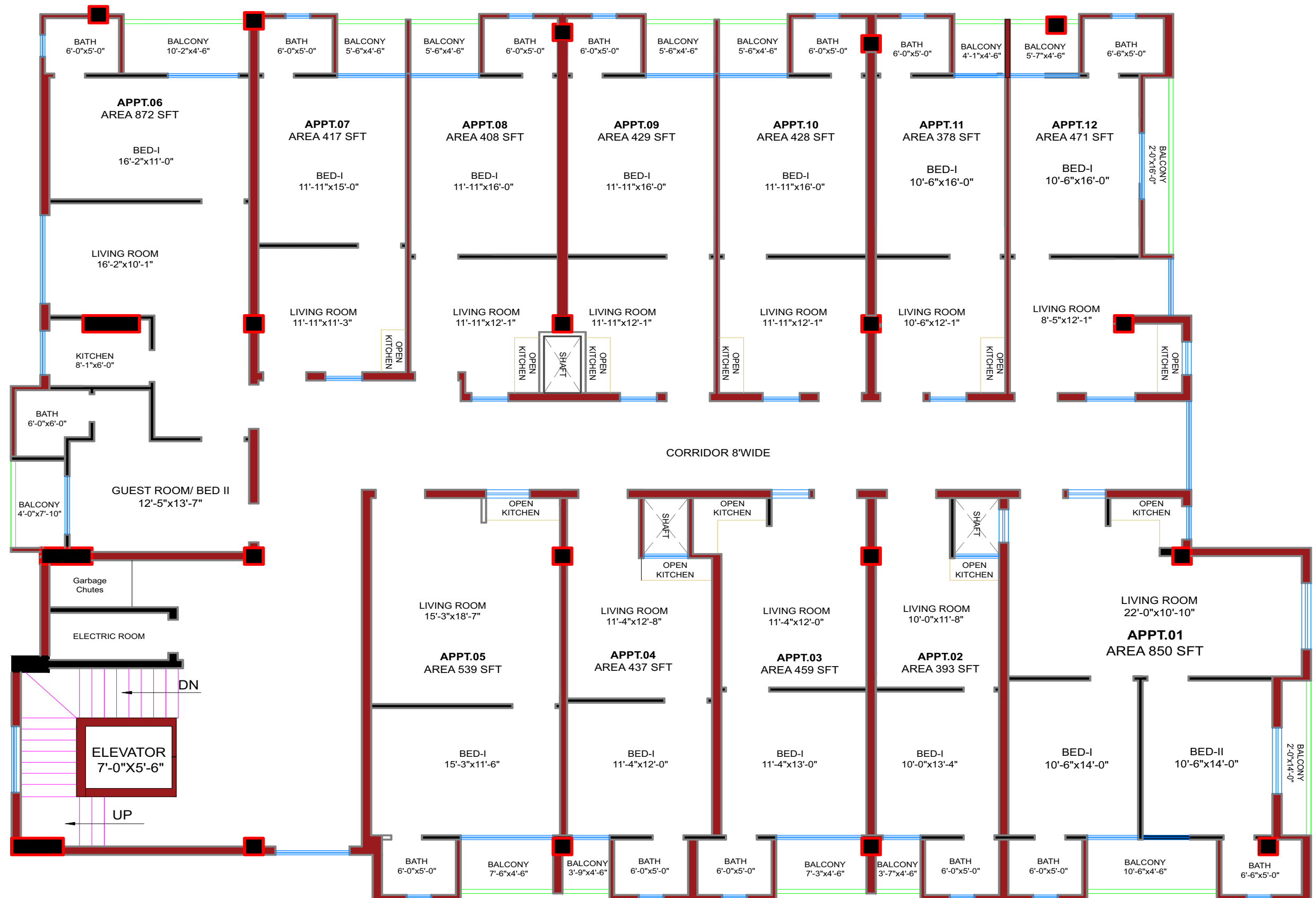
SECOND & THIRD FLOOR PLAN
