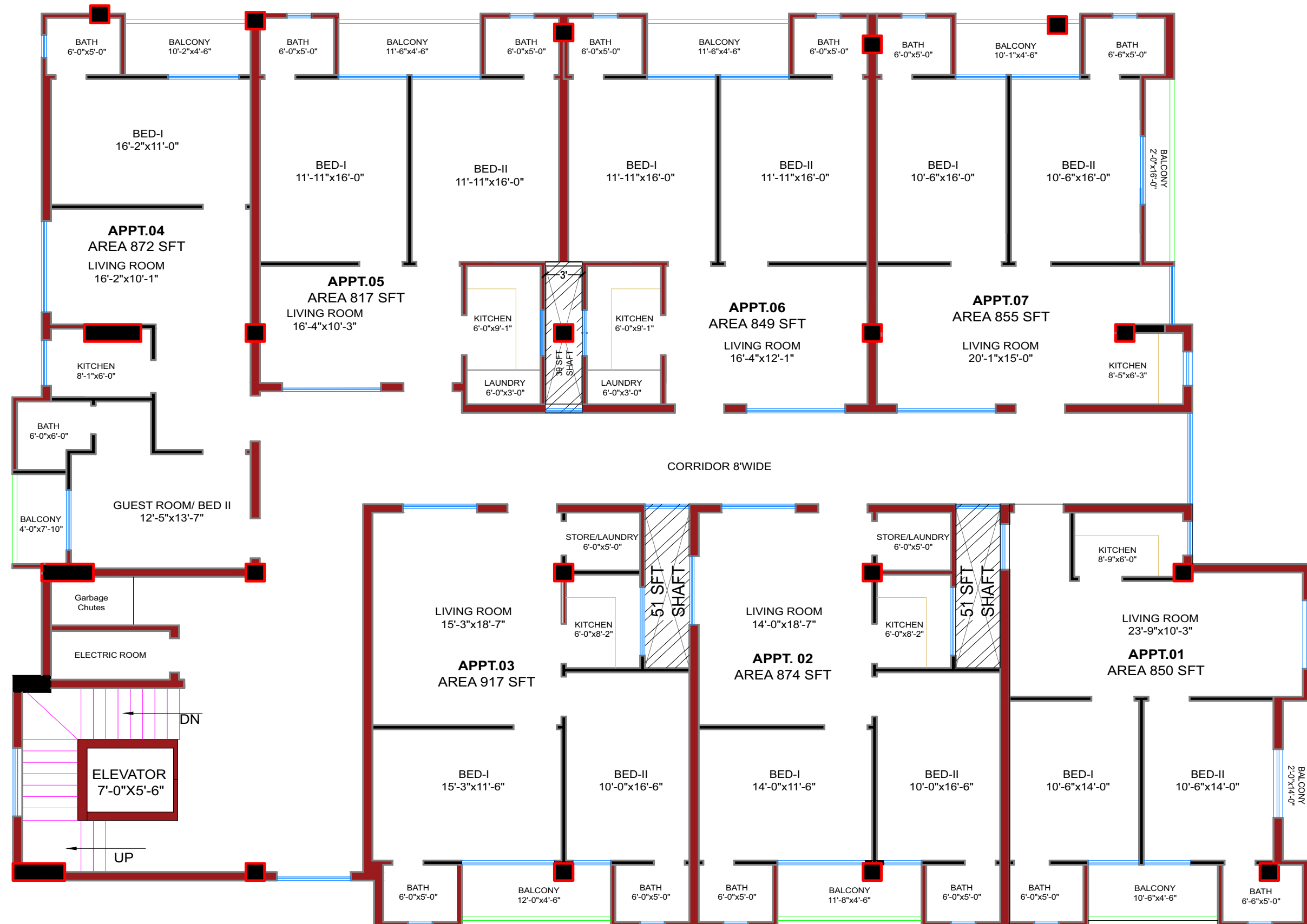
FOURTH TO SIXTH FLOOR PLAN
